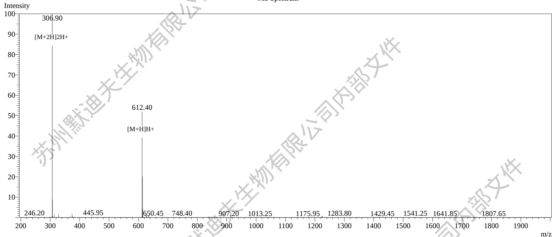
MS Spectrum
