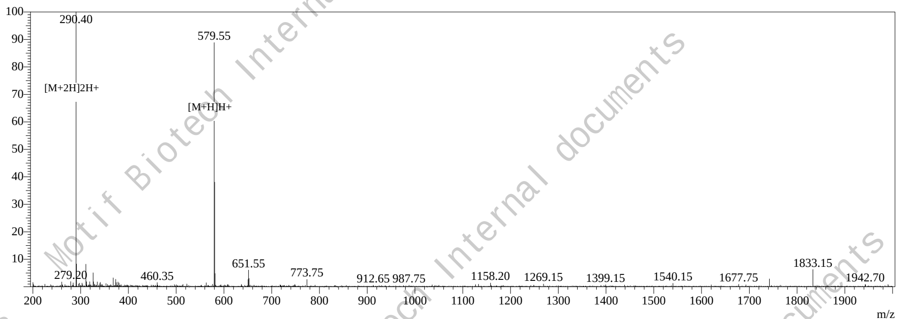
MS Spectrum
