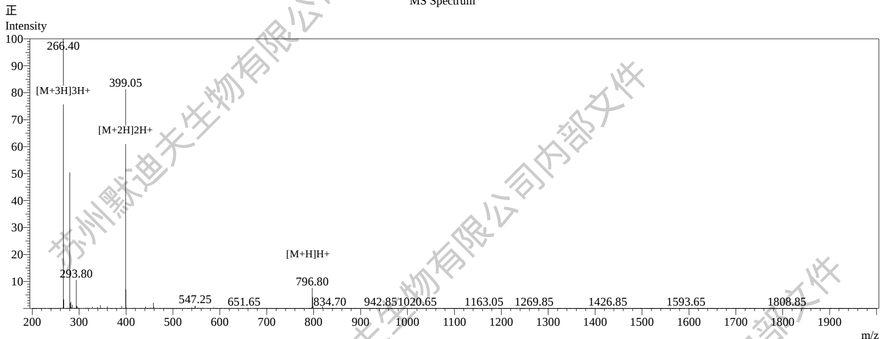
MS Spectrum
